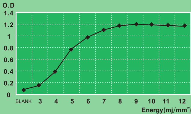
DYNAMIC SENSITIVITY
